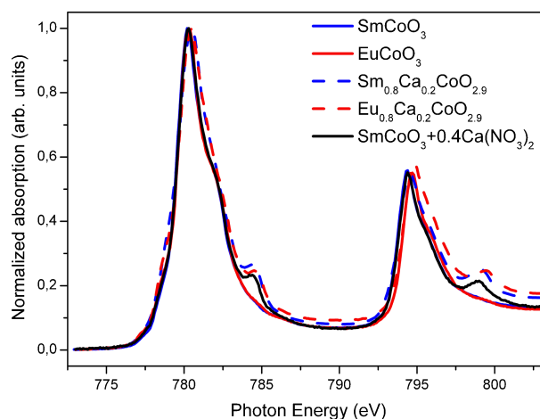
Fig. 4. (Color online) The Co L_{2,3} -edge XANES spectra in \text{EuCoO}_3 , \text{SmCoO}_3 , \text{Eu}_{0.8}\text{Ca}_{0.2}\text{CoO}_{2.9} , \text{Sm}_{0.8}\text{Ca}_{0.2}\text{CoO}_{2.9} , and in the mechanical mixture of \text{SmCoO}_3 and 0.4\text{Ca}(\text{NO}_3)_2 powders.
