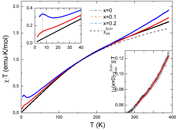
Fig. 7. (Color online) The temperature dependences of the product \chi \cdot T for the \text{Eu}_{1-x}\text{Ca}_x\text{CoO}_{3-\delta} family of compounds. Lower inset represents the difference between the data for x = 0 and the \text{Eu}^{3+} van Vleck contribution (black data and dashed line, respectively, in main plot). The upper inset highlights the low temperature behavior.
