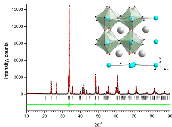
Fig. 1. (Color online) Room temperature powder XRD pattern (black circles) of \text{EuCoO}_3 in the 2\theta range 10–90°, Rietveld refinement fit (upper solid line), difference profile (lower solid line), and positions of Bragg peaks (vertical bars). In the inset the primitive cell of \text{EuCoO}_3 is shown. The Eu ions are indicated by large gray circles, the Co ions both bare and in octahedral oxygen environment are represented by blue circles and two positions of oxygen ions are shown by small red (O1) and black (O2) circles.
