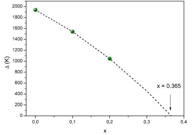
Fig. 8. (Color online) The concentration dependence of the gap \Delta between low spin and intermediate spin states in the \text{Eu}_{1-x}\text{Ca}_x\text{CoO}_{3-\delta} family of compounds. The dashed line is a polynomial extrapolation of the experimental data.
