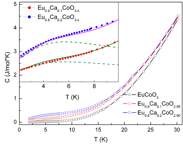
Fig. 5. (Color online) The temperature dependences of specific heat C in \text{Eu}_{1-x}\text{Ca}_x\text{CoO}_{3-\delta} series of compounds. Inset: the approximation of the specific heat in Ca-doped compounds by sum of cubic term \beta T^3 (not shown) and Schottky-type anomaly C_{\text{Sch}} (dashed lines).
