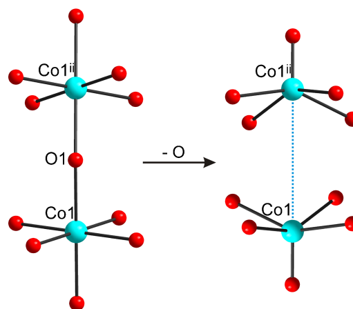
Fig. 2. (Color online) The scheme of local environment of two neighboring \text{Co}^{3+} ions in octahedral and pyramidal coordination.
