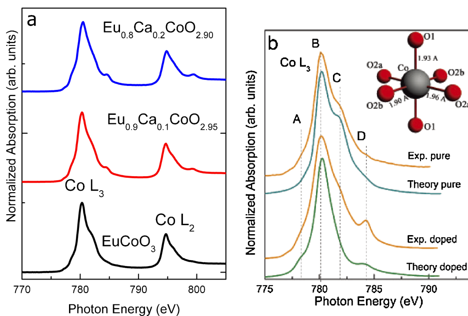
Fig. 3. (Color online) The Co L_{2,3} -edge XANES spectra in \text{Eu}_{1-x}\text{Ca}_x\text{CoO}_{3-\delta} series of compounds taken at liquid nitrogen temperature (a); the comparison of experimental and simulated XANES spectra in pure \text{EuCoO}_3 and Ca-doped compounds (b). The inset shows the nearest coordination of the Co atom together with the corresponding bond distances. The spectra were shifted along y-axis for clarity.
